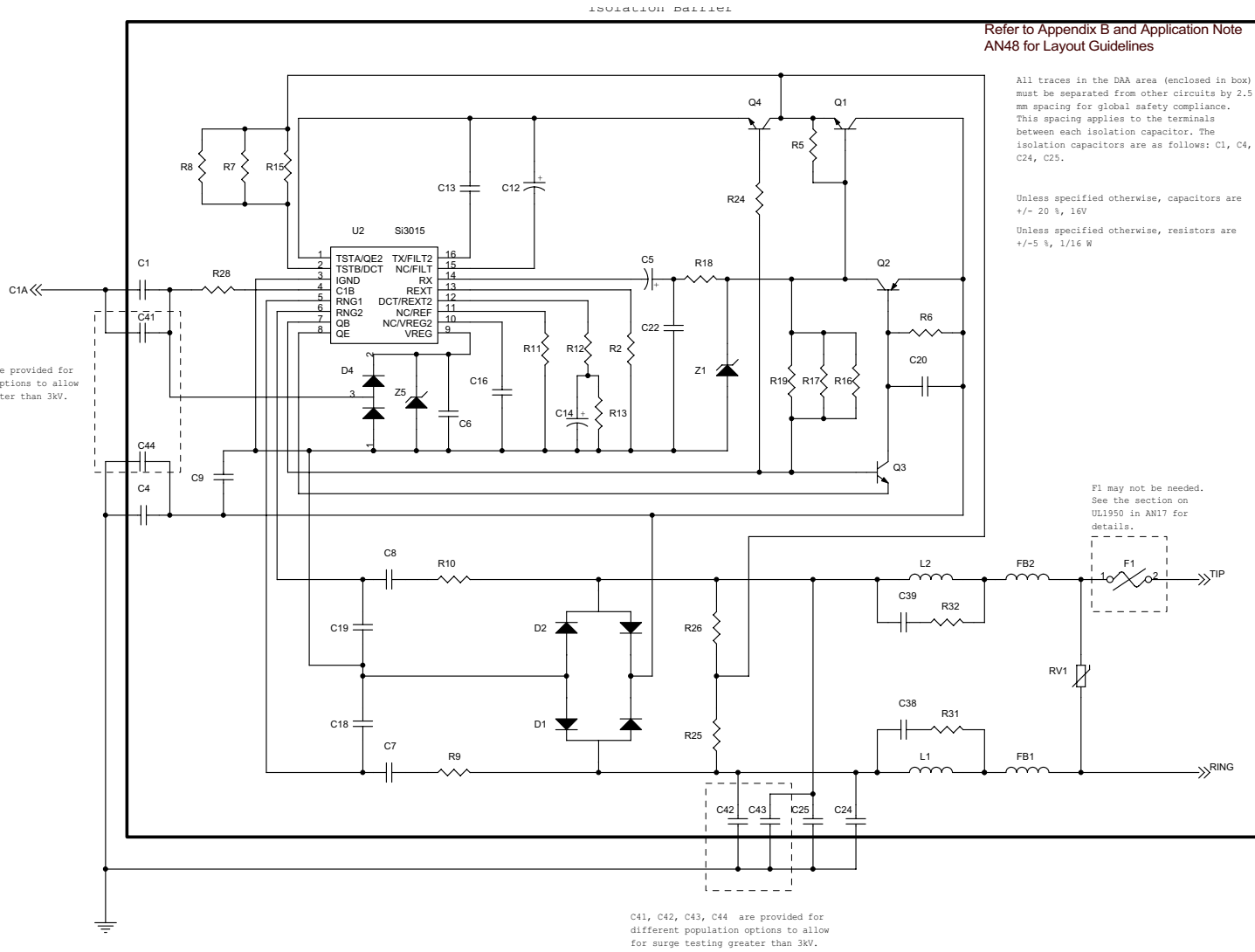
Figure 4. Si3015 DAA Schematic
