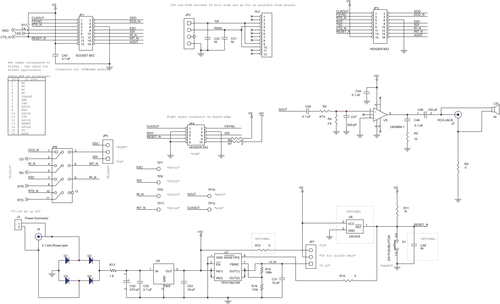
Figure 6. Si2400URT-EVB Motherboard Power, Connector, Audio Schematic
