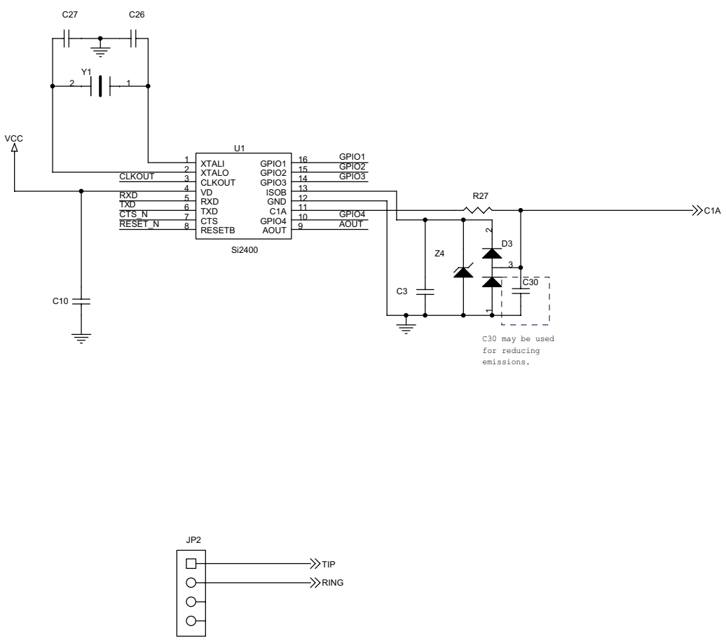
Figure 3. Si2400 Schematic
